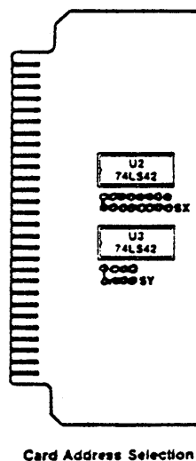
FIGURE 3 - DECODER JUMPER PAD NUMBERING
