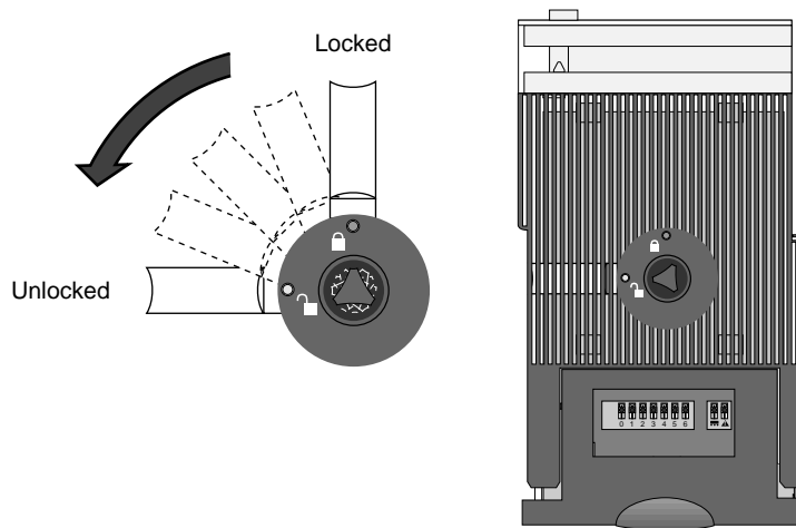
Figure 33. Unlocking the HDDA drive drawer
