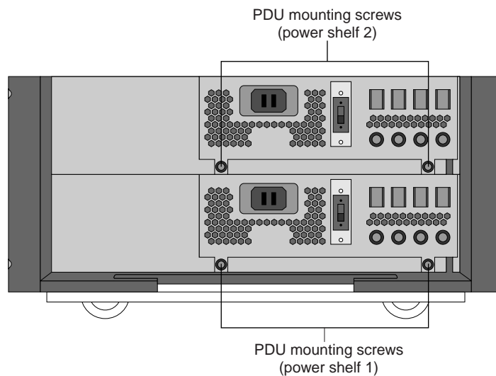
Figure 27. PDU mounting screw locations
