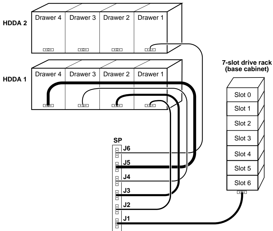
Figure 44. Example SCSI cabling for NS 7000/030 (back view)
