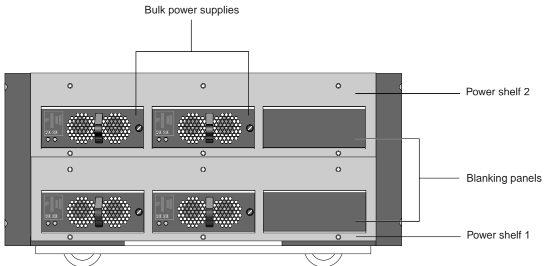
Figure 24. Location of Power Supplies
