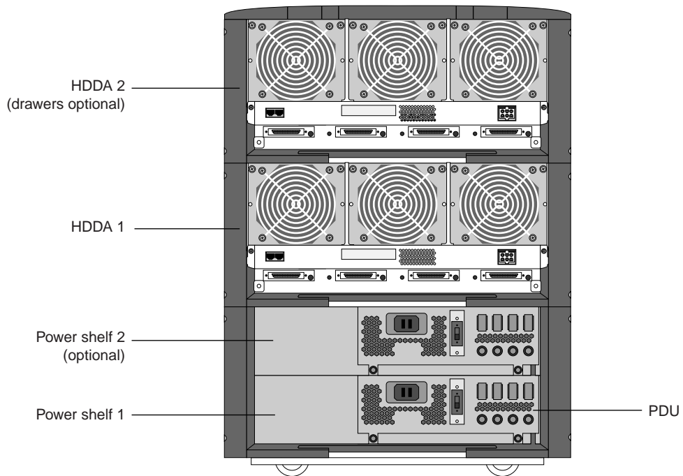
Figure 2. NS 7000/030 storage subsystem (back view)
