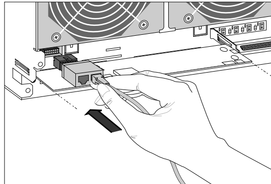
Figure 46. Installing the HDDA monitoring board
