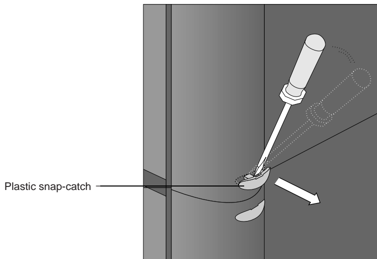
Figure 29. Removing the plastic snap-catch
