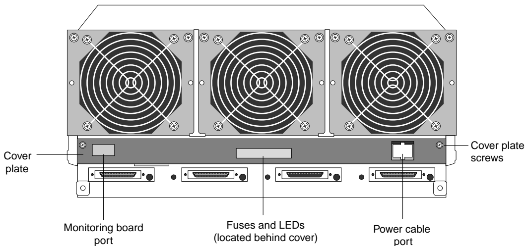
Figure 21. Drawer fuses and LEDs location (HDDA back view)
