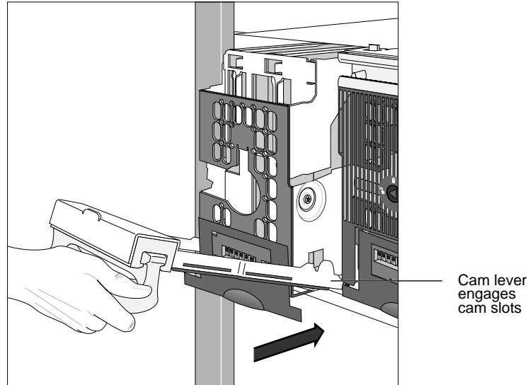
Figure 16. Installing a drive drawer
