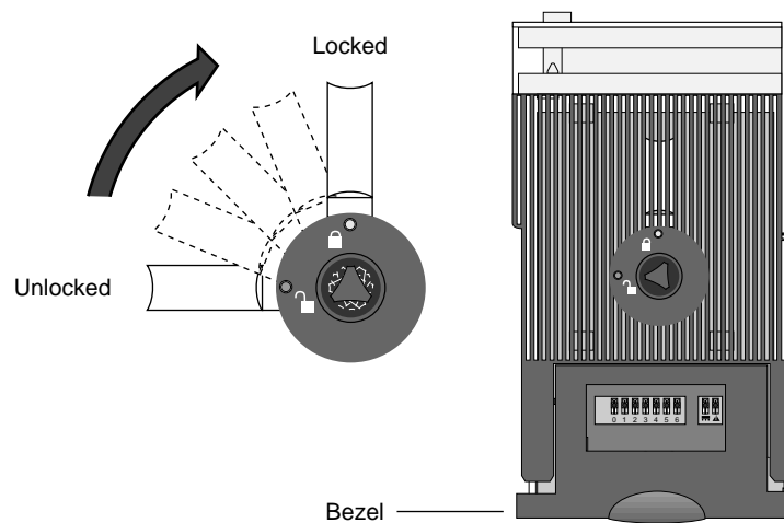
Figure 41. Locking the HDDA drive drawer
