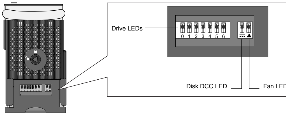
Figure 32. Disk DCC LED (drive drawer front panel)
