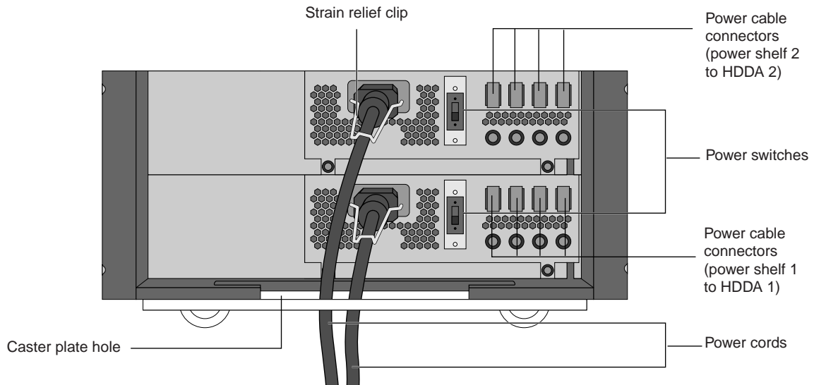
Figure 26. NS 7000/030 power system (back view)
