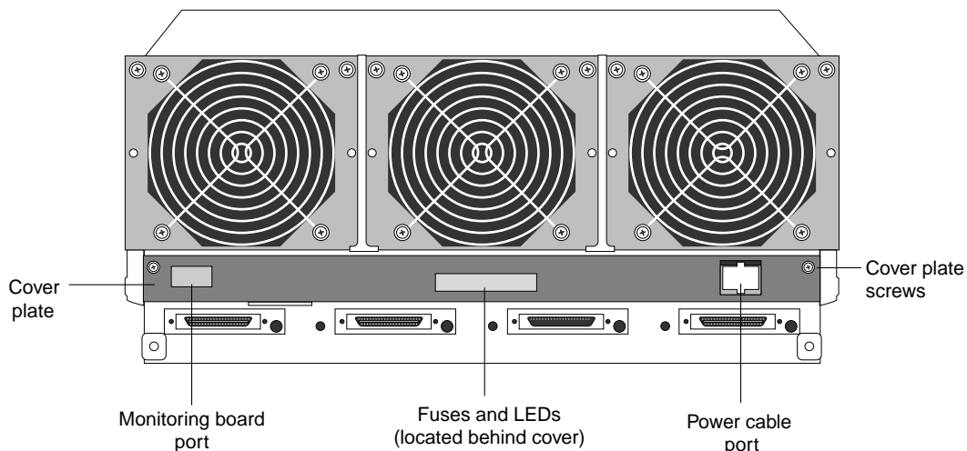
Figure 3. Rear cover plate and power cable cutout
