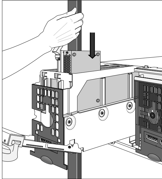
Figure 37. Inserting the Disk DCC
