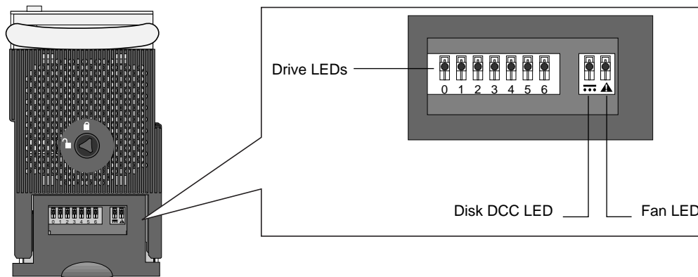
Figure 42. Location of fan LED
