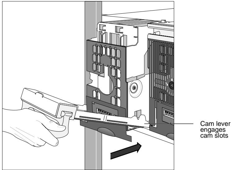
Figure 38. Closing the HDDA drive drawer
