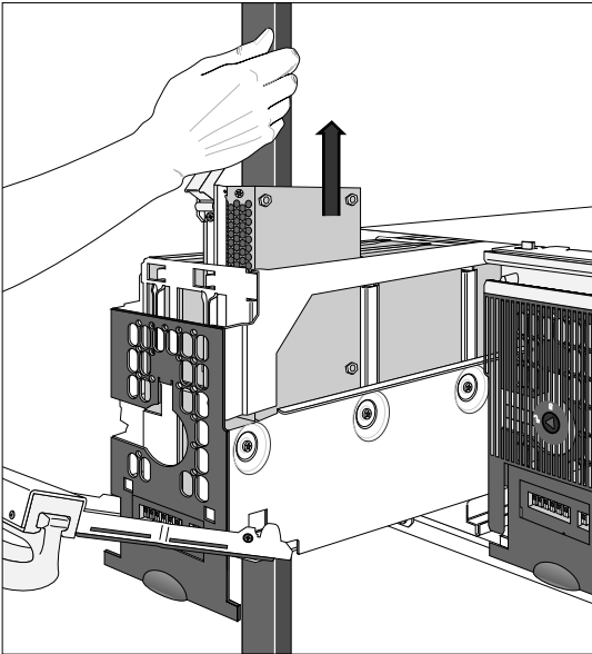
Figure 36. Removing the Disk DCC
