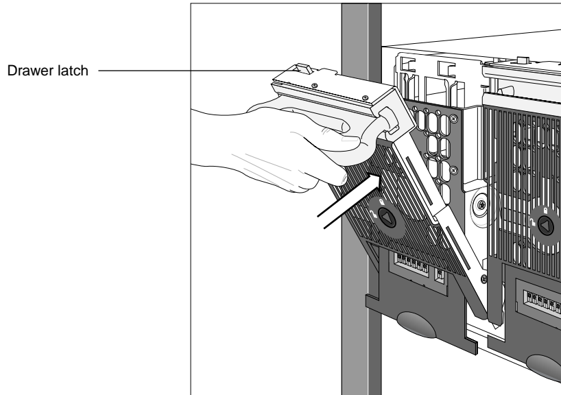
Figure 18. Closing a drive drawer
