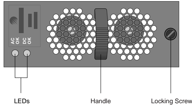
Figure 25. Bulk power supply LEDs
