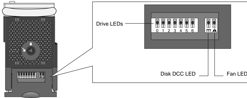
Figure 20. HDDA LEDs (drive drawer front panel)
