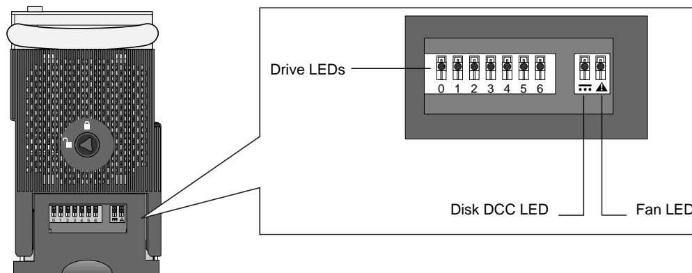
Figure 7. Drive drawer LEDs (drive drawer front panel)
