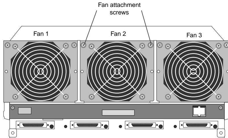
Figure 43. Location of HDDA fans (back of HDDA chassis)
