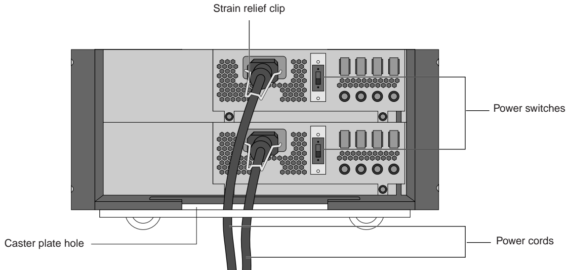
Figure 28. Bulk power supply chassis (back)
