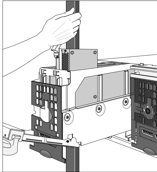
Figure 15. Removing and Replacing the Disk DCC
