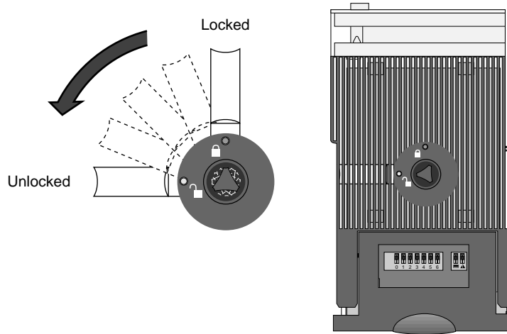
Figure 22. Unlocking the HDDA drive drawer
