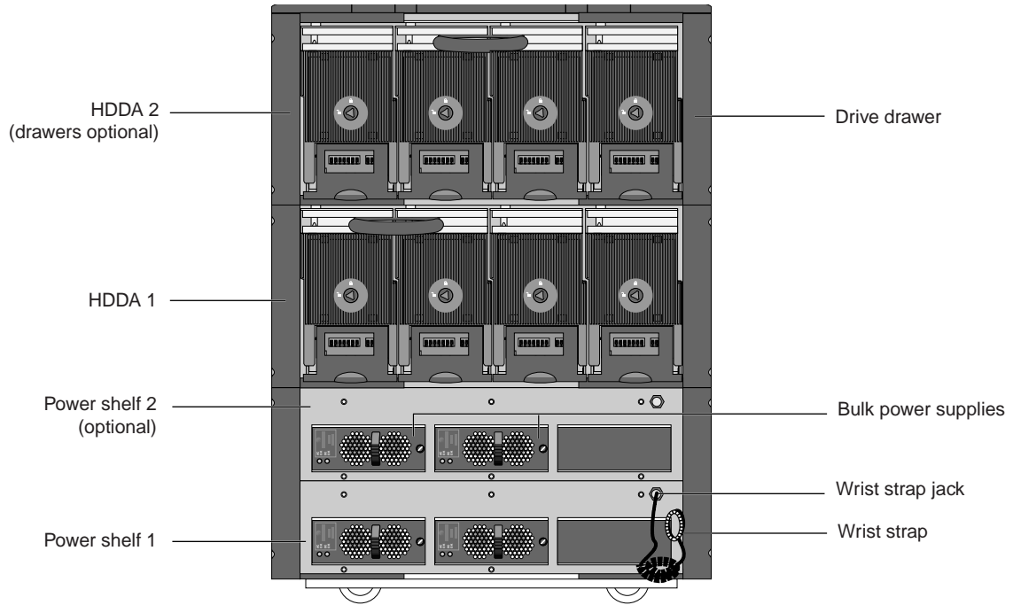
Figure 1. NS 7000/030 storage subsystem (front view)
