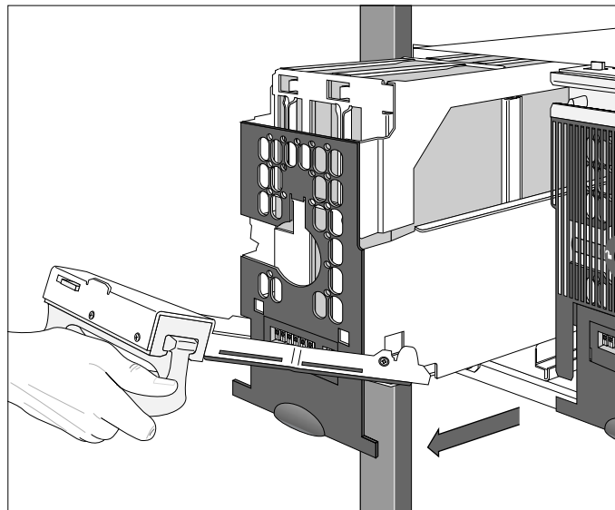
Figure 23. Opening the drive drawer
