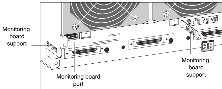
Figure 45. HDDA monitoring board location
