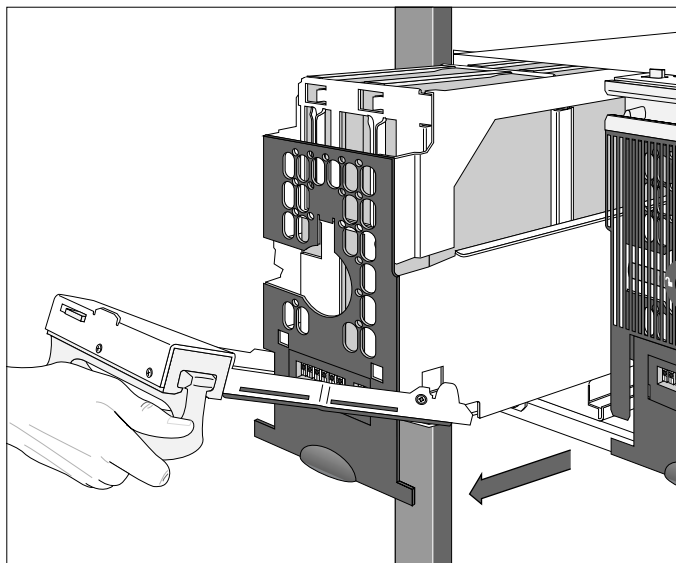
Figure 34. Opening the drive drawer
