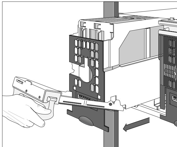
Figure 13. Removing an HDDA drive drawer
